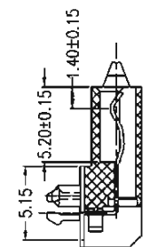
SECT B-B
