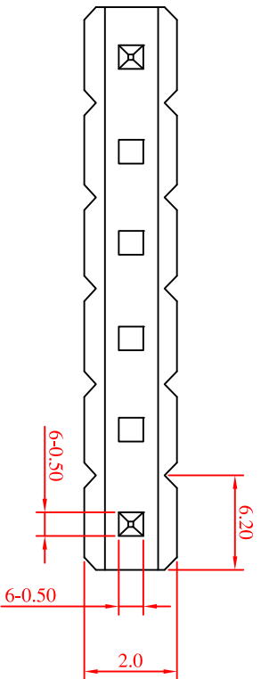
Pin Chart
