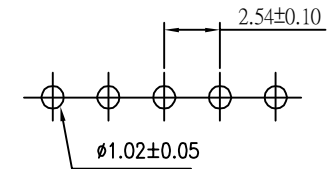
Recommended P.C. Board Hole Layout
