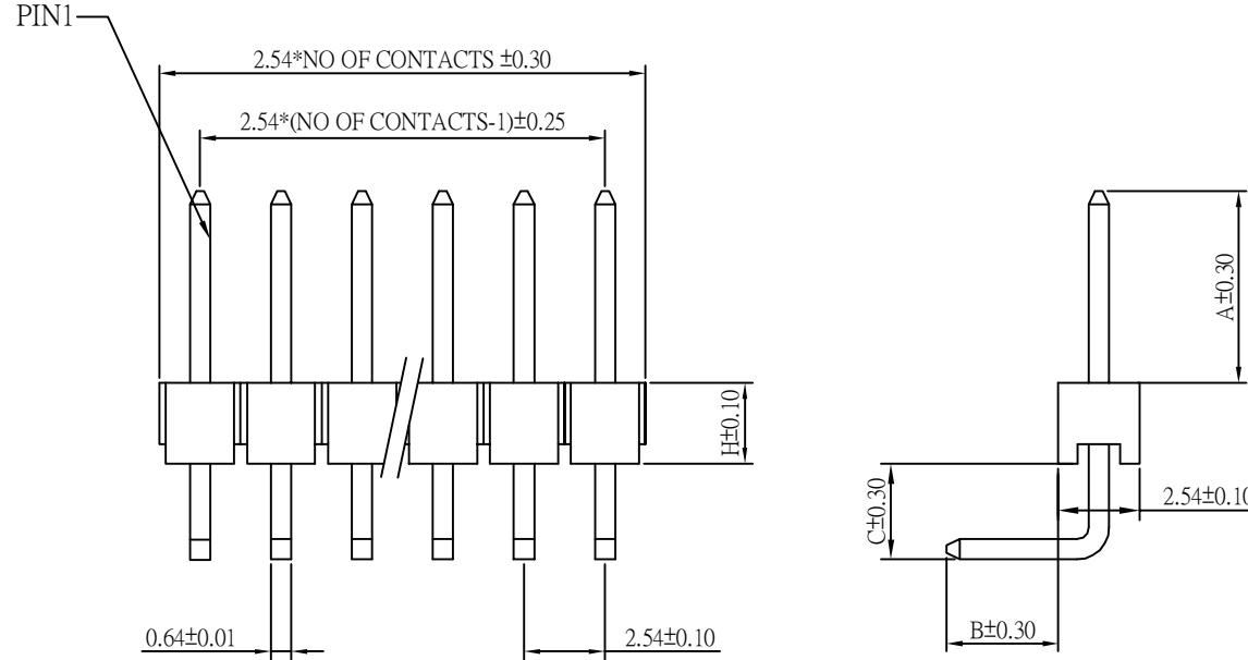
Pin Chart
