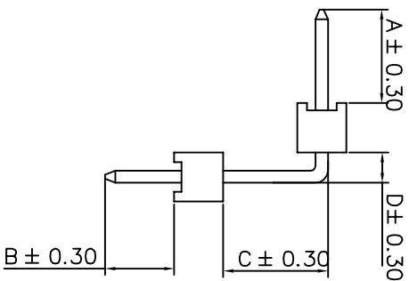
Pin Chart
